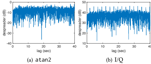
Figure 9: Low SNR regime comparison between (a) real despreaders after atan2 demapping, and (b) complex despreaders operating on I/Q directly.
